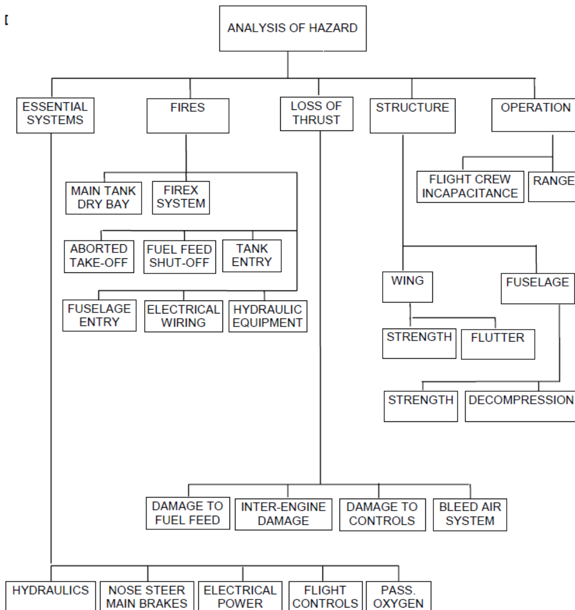
EXAMPLE – HAZARD TREE
