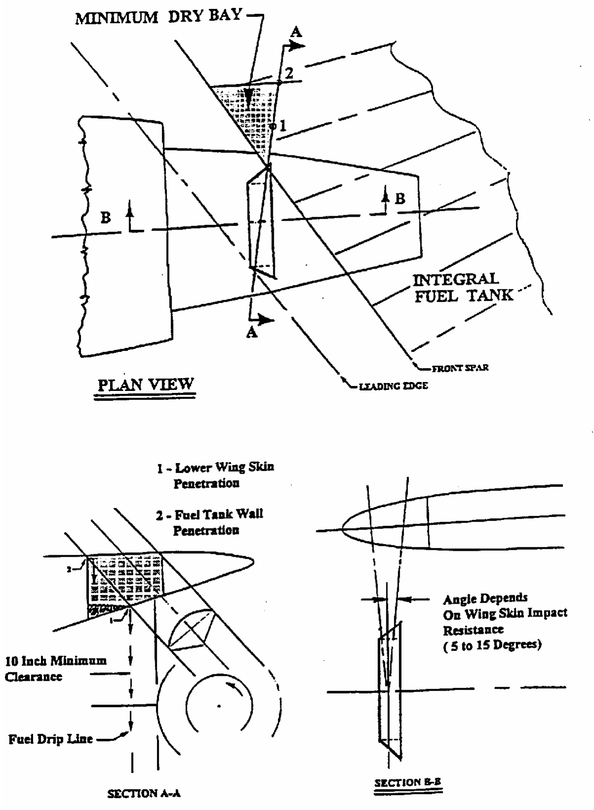
FIGURE 2 – DRY BAY SIZING DETERMINATION EXAMPLE
