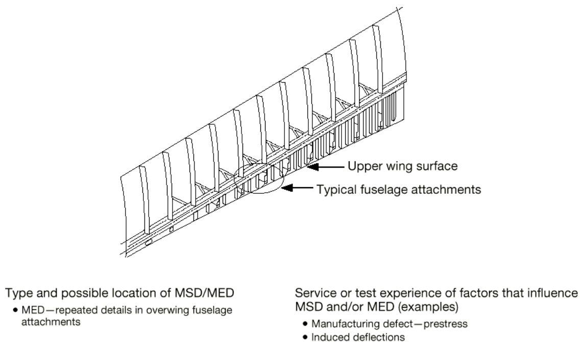
Figure A2-11 Over Wing Fuselage Attachments (MED)
