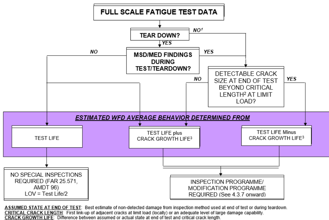
Figure A2-18 Use of Fatigue Test and Teardown Information to Determine WFD Average Behaviour
